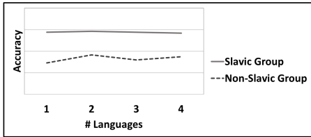
Figure 2: Slavic Accuracy
