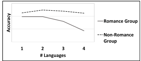
Figure 3: Romance Accuracy
